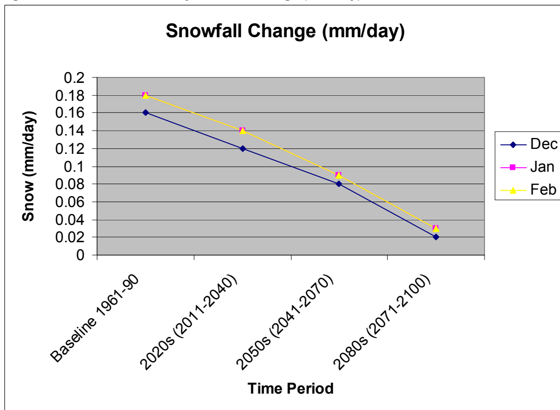
Figure A10: Predicted monthly snowfall change (mm/day)
