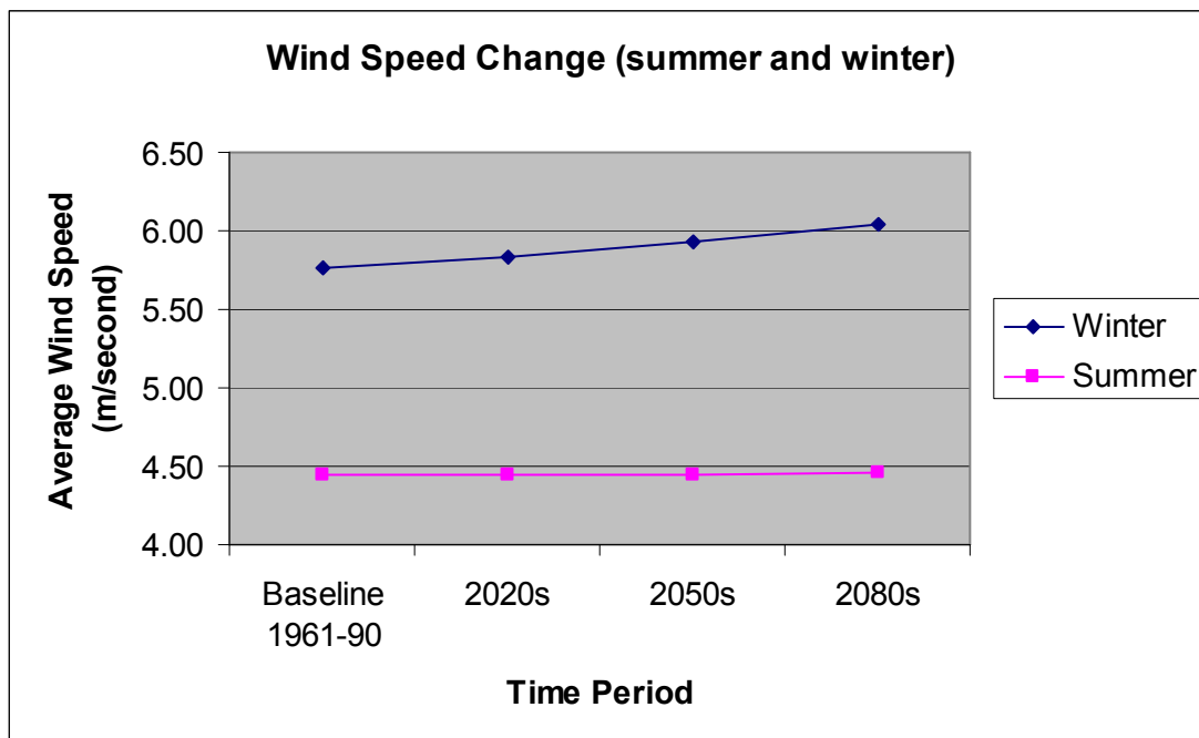
Figure A9: Average winter and summer wind speed change (m/second)
