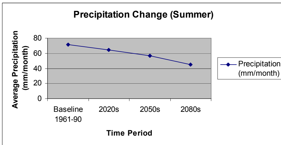
Figure A3: Average summer precipitation change
