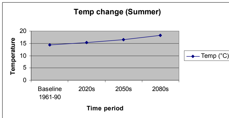
Figure A6: Average summer temperature change (°C)
