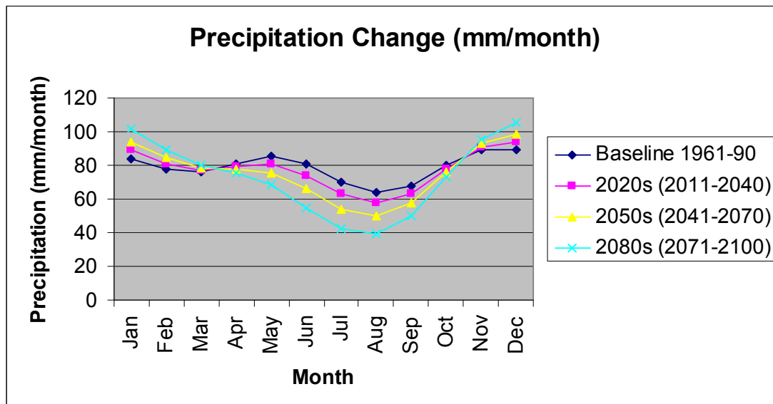
Figure A2: Precipitation change (mm/month)
