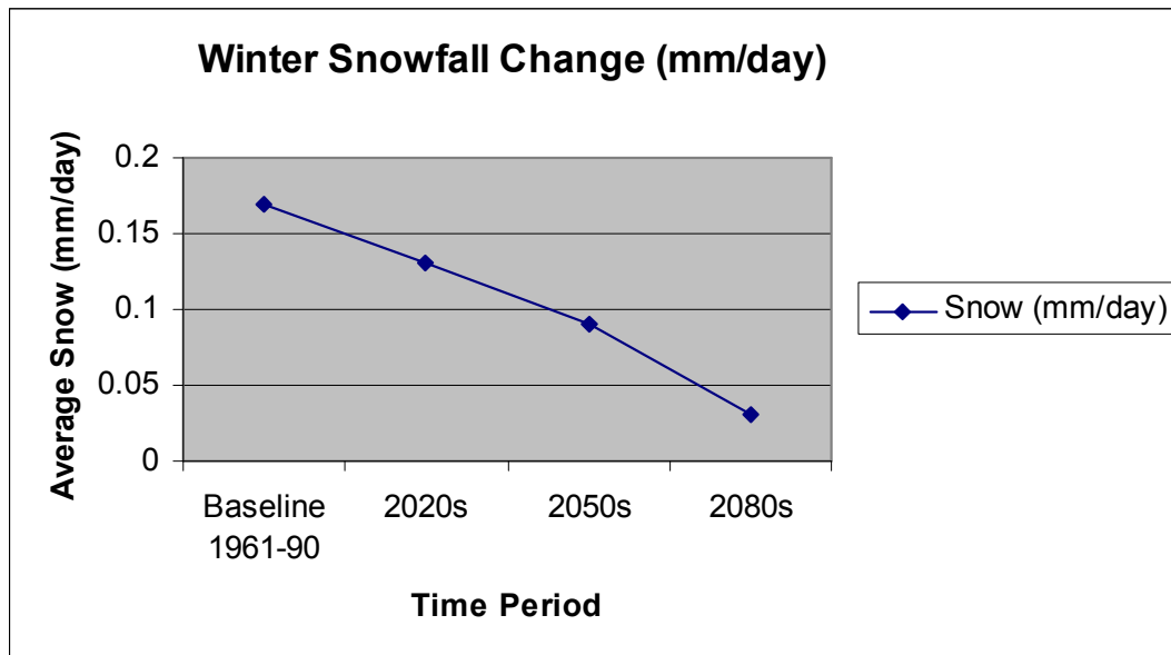
Figure A11: Predicted average winter snowfall change (average over Jan, Feb and March), (mm/day)
