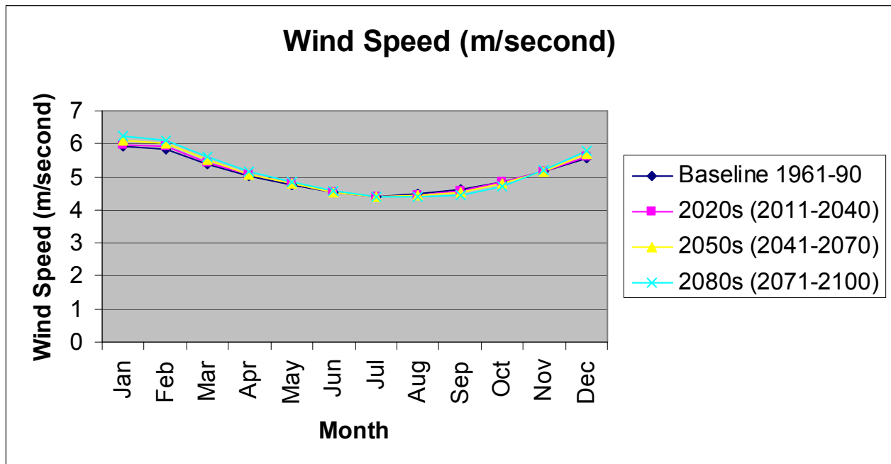
Figure A8: Wind speed change
