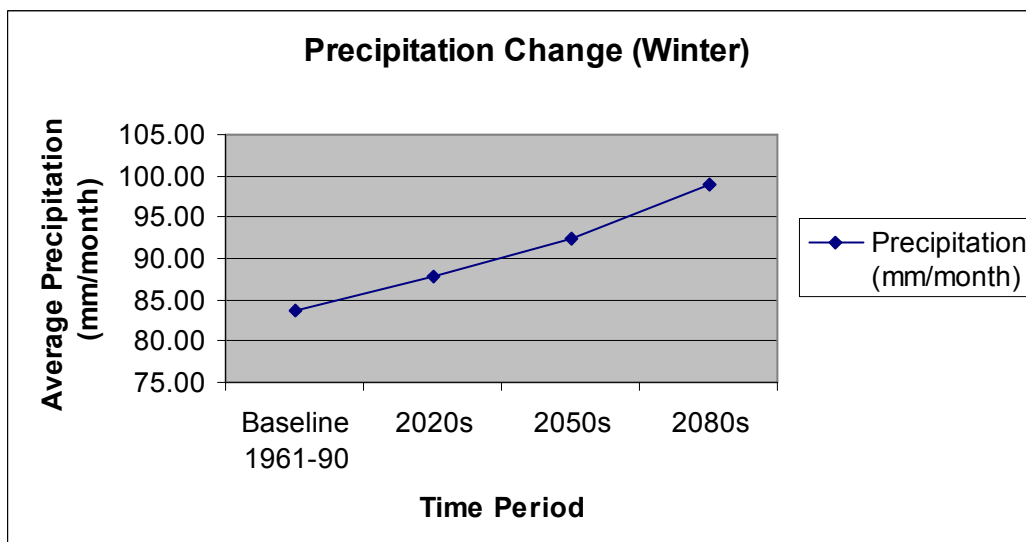
Figure A4: Average winter precipitation change
