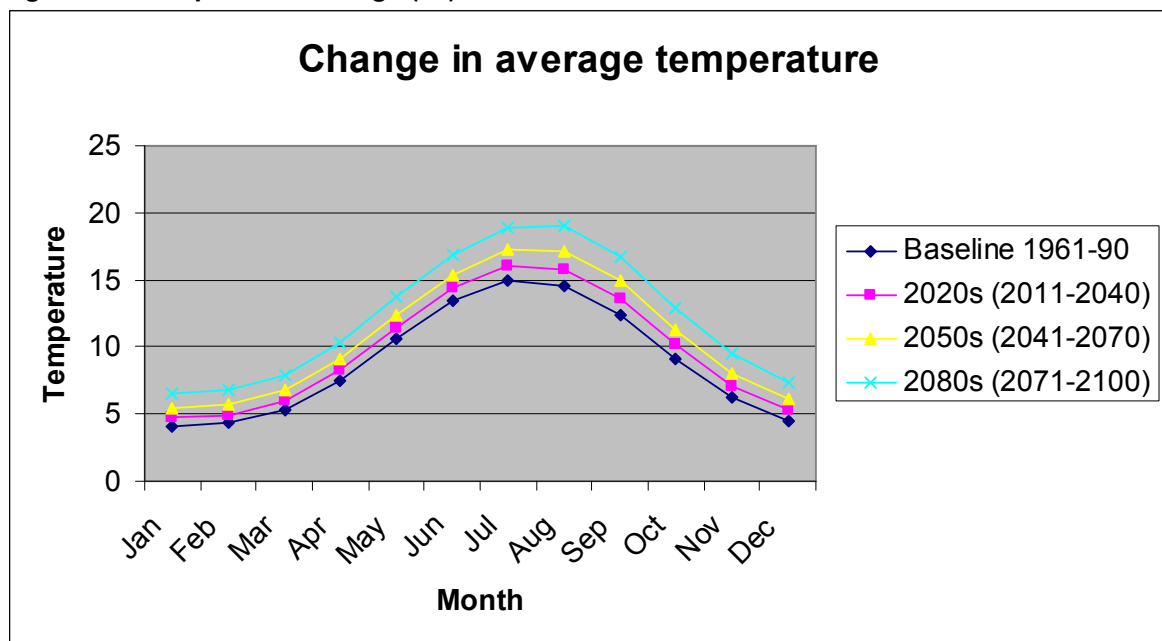
Figure A5: Temperature change (°C)
