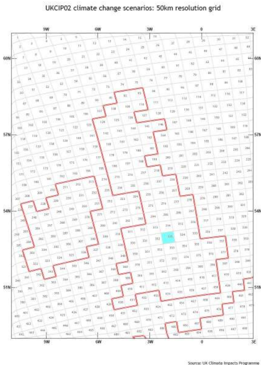
Figure A1: UKCIP Climate Scenarios 50km grid – showing selected grid square 333
